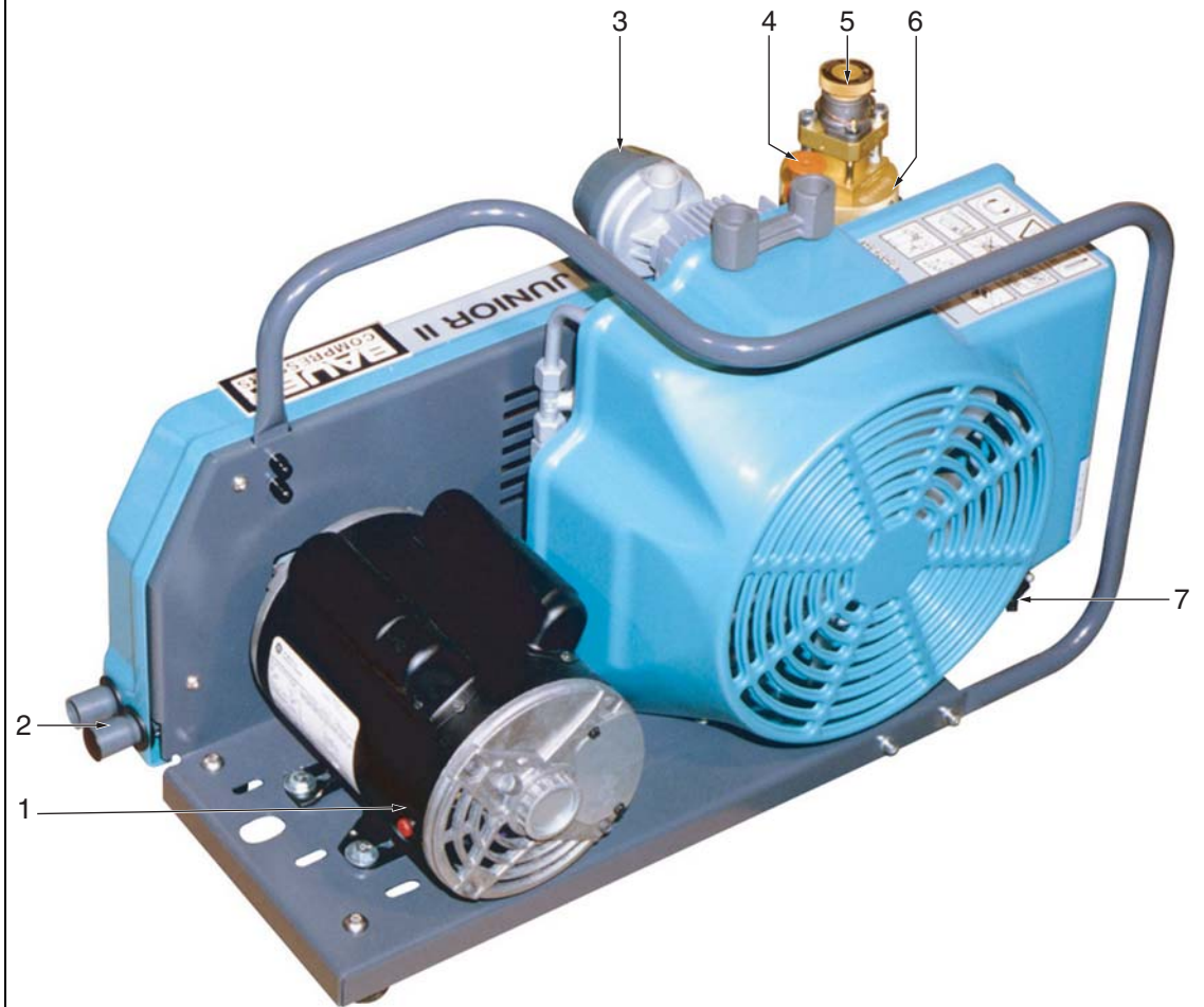
Figure 1-1 Junior II with Single Phase Electric Motor
